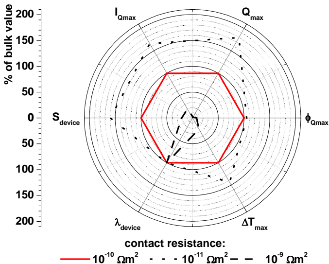
Figure 2. Performance qualification plot for different contact resistances, thermocouple height = 20\mu\text{m}
