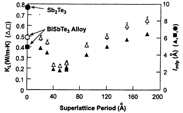
Figure 4. Decrease of lattice thermal conductivity \kappa_L in (Bi,Sb) 2 Te 3 /Sb 2 Te 3 superlattices [24].
