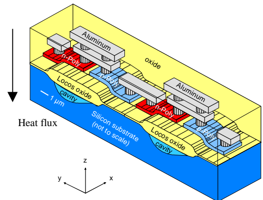
Figure 6. Schematic setup of the Infineon CMOS micro TEC [28].
