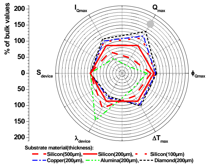
Figure 3. Performance qualification plot for different substrates. ● indicates Q_{\text{max}} for an “ideal” substrate without any thermal resistance
