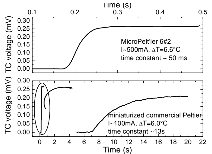
Figure 13. Comparison of the response time of this MicroTEC and the smallest commercially available device for \Delta T of about 6^\circ\text{C} .
