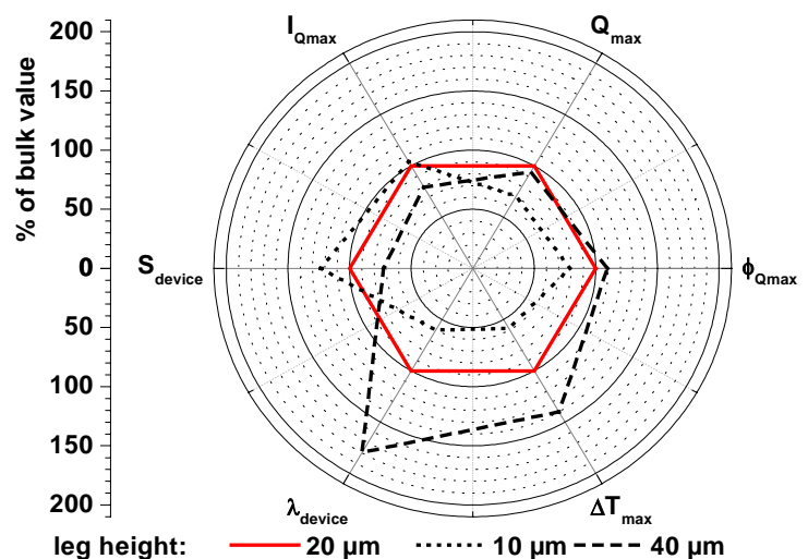
Figure 1. Performance qualification plot for different leg heights.
