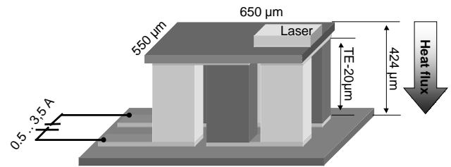
Figure 7. Schematic drawing of a possible telecommunication device
