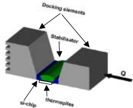
Figure 5. Scheme of the P3F TEC
